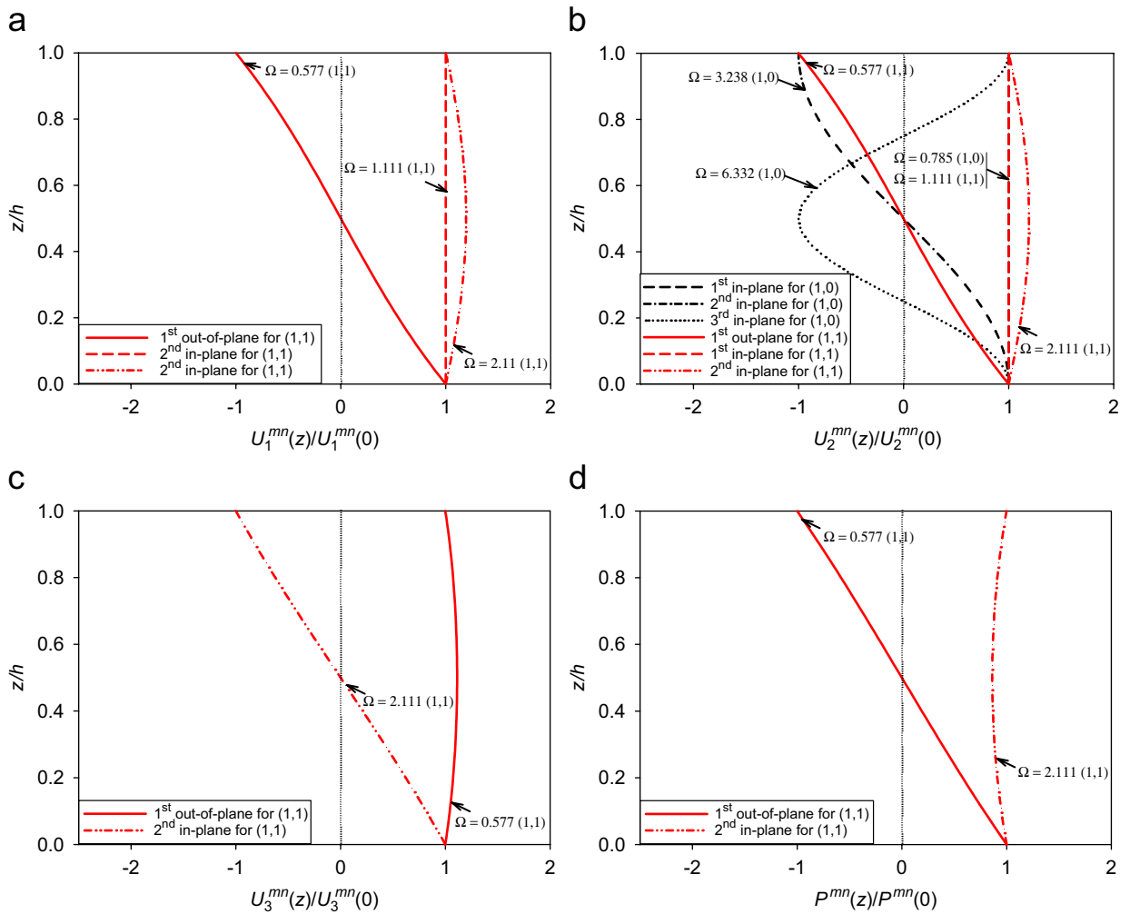
Fig. 1. For (m, n) = (1, 0) and (1, 1) through-the-thickness variation of the normalized displacement components and the pressure for three thickness modes of vibration. (a) —1st out-of-plane for (1, 1) , \Omega = 0.577 ; ----2nd in-plane for (1, 1) , \Omega = 1.11 ; and -·-·-2nd in-plane for (1, 1) , \Omega = 2.11 ; (b) ---- 1st in-plane for (1, 0) , \Omega = 3.238 ; -·-·-2nd in-plane for (1, 0) , \Omega = 0.785 ; ·····3rd in-plane for (1, 0) , \Omega = 6.332 ; —1st out-of-plane for (1, 0) , \Omega = 0.577 ; ----1st in-plane for (1, 0) , \Omega = 1.111 ; and -·-·-2nd in-plane for (1, 0) , \Omega = 2.111 ; (c) —1st out-of-plane for (1, 1) , \Omega = 2.111 and -·-·- 2nd in-plane for (1, 1) , \Omega = 0.577 ; and (d) —1st out-of-plane for (1, 1) , \Omega = 0.577 and -·-·-2nd in-plane for (1, 1) , \Omega = 2.111 .
